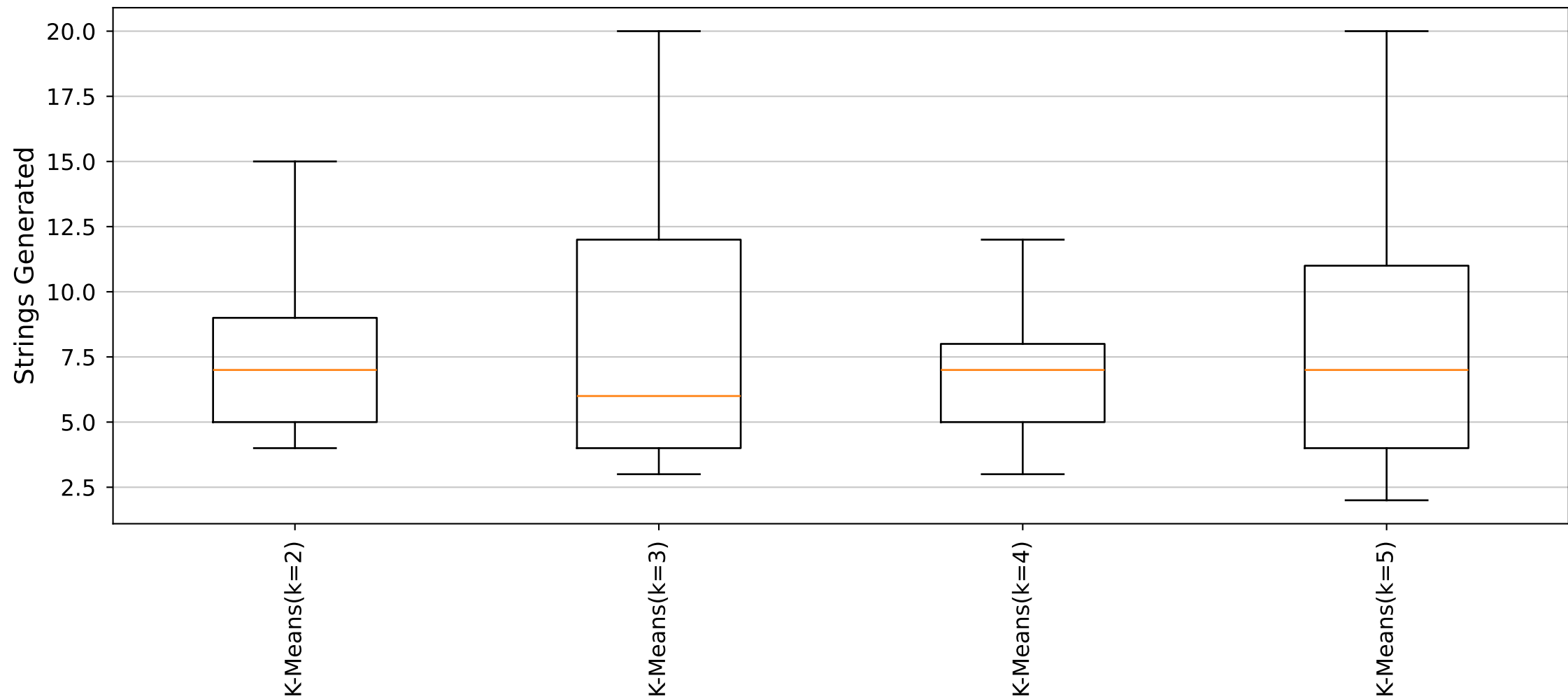
YARA Rules Strings Generated Distribution (Cluster45_Size5 dataset)
